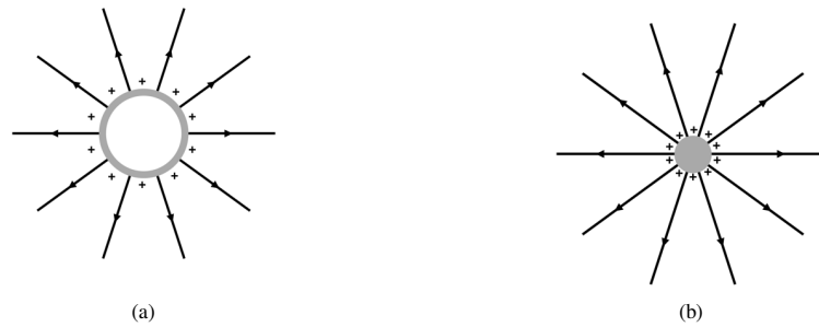
Fig. 1. (a) The electric field pulls outward on the sphere. (b) If the sphere is compressed while the charge is held constant, new field is created. For this, energy has to be supplied to the system.
