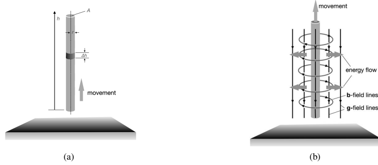
Fig. 3. (a) A rod is pulled from the top. In the process, energy flows within the rod from top to bottom. (b) This energy gradually leaves the rod sideways.
