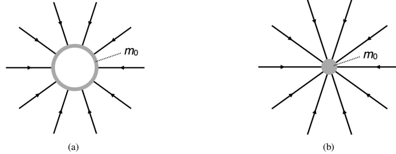
Fig. 2. (a) The gravitostatic field pushes on the sphere. (b) If the sphere is allowed to shrink with the mass kept constant, new field is created. For this, energy has to be removed from the system.
