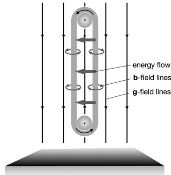
Fig. 4. In the left part of the rope, the energy flows within the rope upward, in the right part downward. In the process, its current strength increases upwards in the left part and decreases downwards in the right part. The circuit is closed by the gravitational field in which the energy flows from the right to the left part of the rope.
