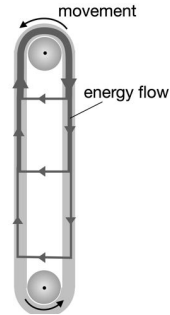
Fig. 5. Energy flow corresponding to Figure 4, schematically
